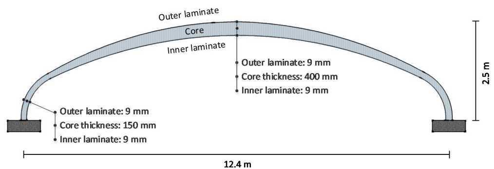
Figure 9. Cross-sectional dimensions of the FRP sandwich shell.
